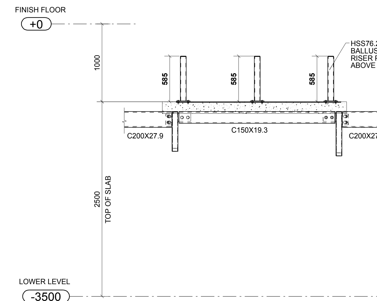
A SECTION
