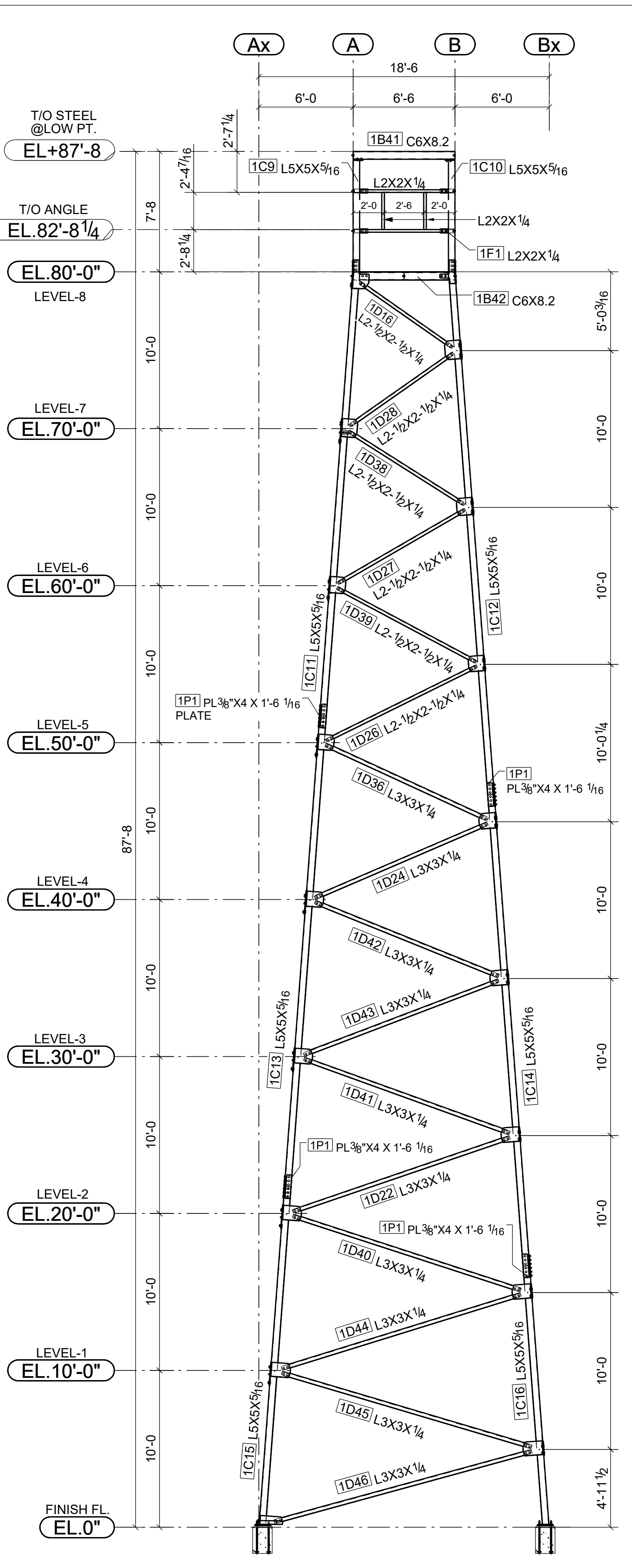
ELEVATION ALONG GRID LINE '2' REFER SHEET:2/S102
