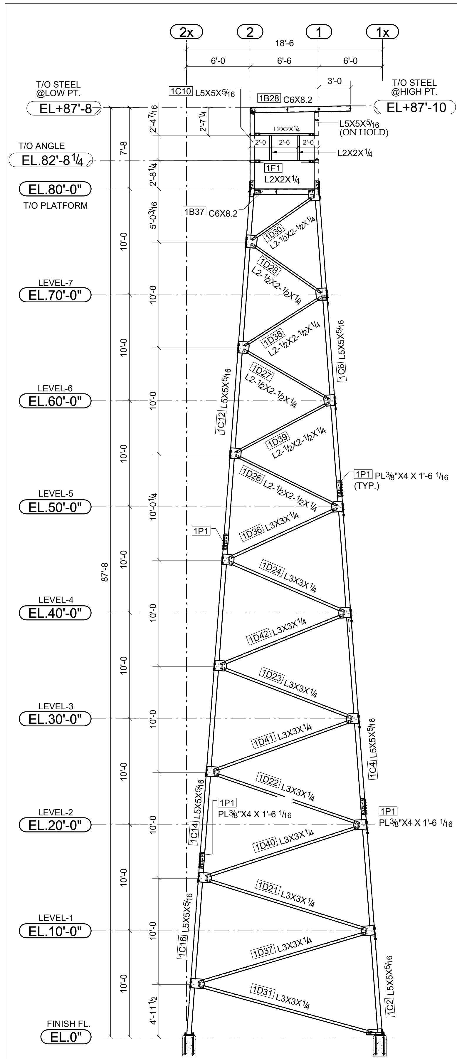
ELEVATION ALONG GRID LINE 'B' REFER SHEET:4/S102
