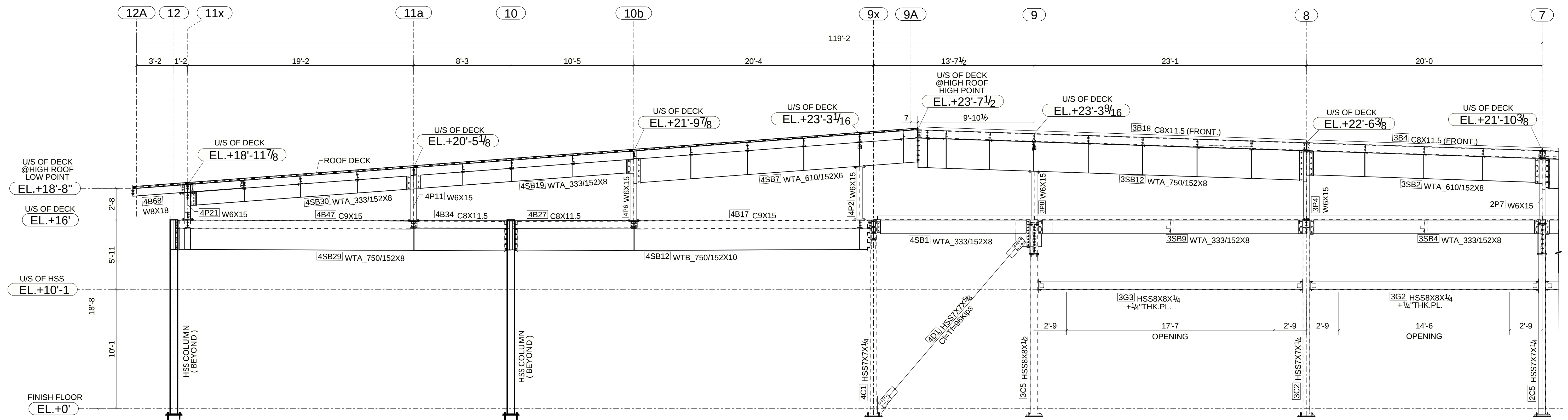
PARTIAL ELEVATION ALONG GRIDLINE 'E' (REFER SHEET : S401)
