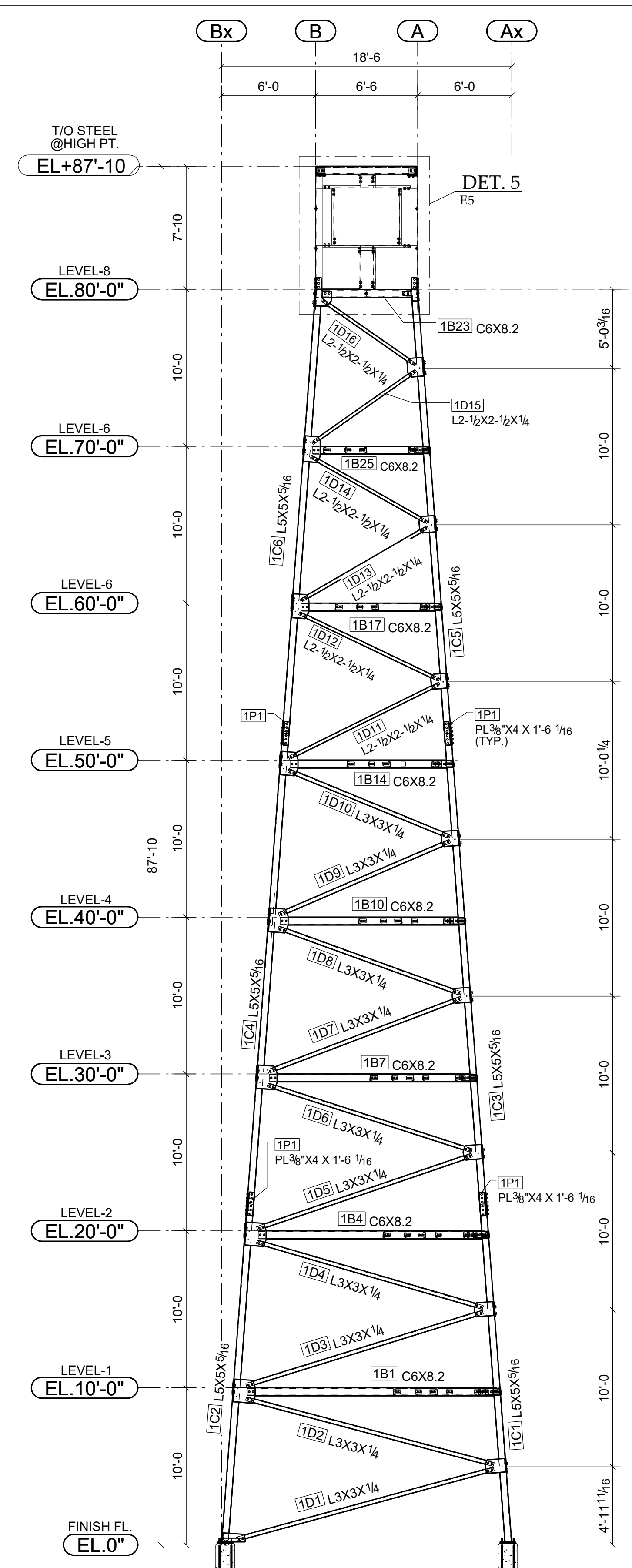
ELEVATION ALONG GRID LINE '1' REFER SHEET:1/S102
