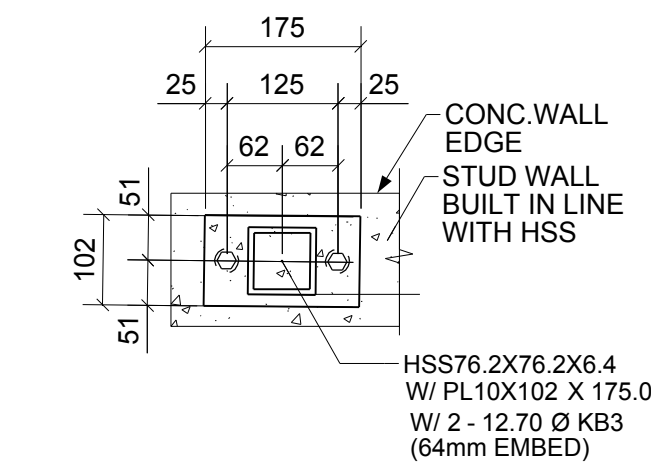
A SECTION
