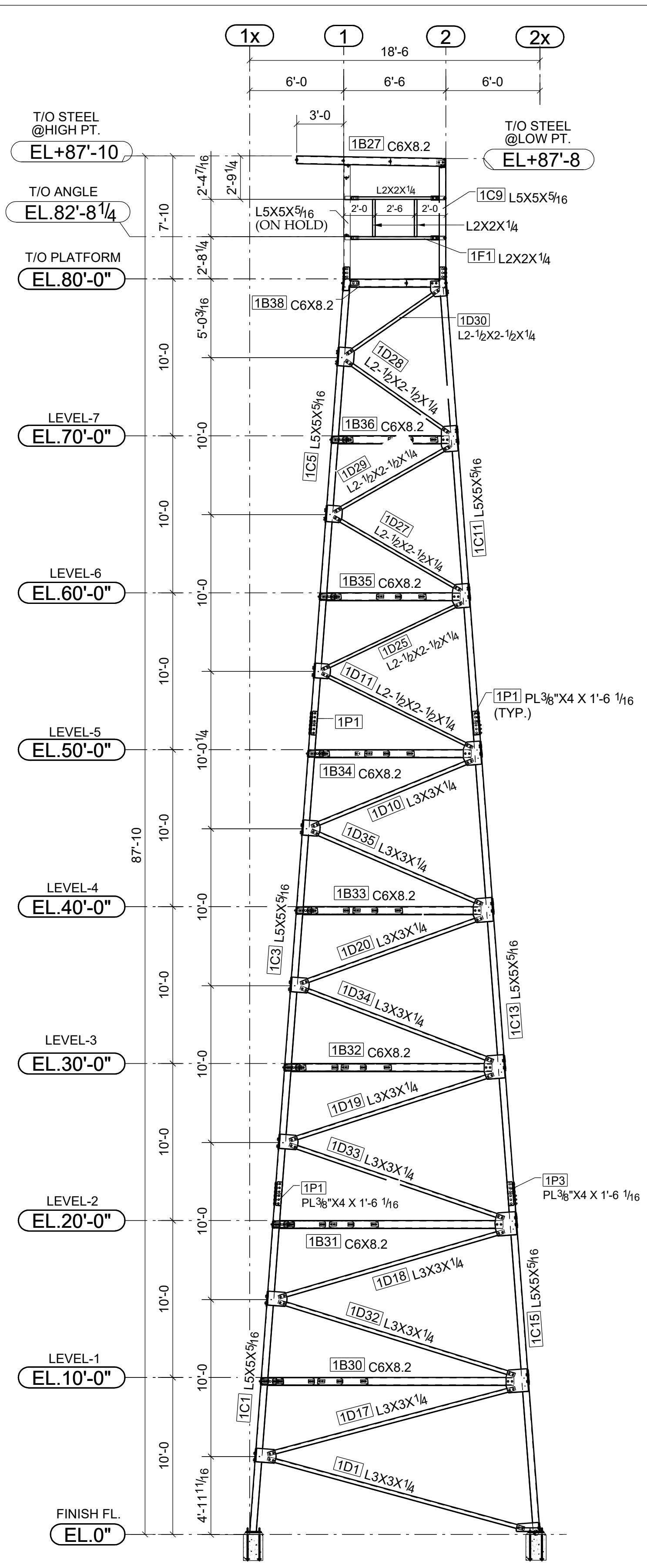
ELEVATION ALONG GRID LINE 'A' REFER SHEET:3/S102
